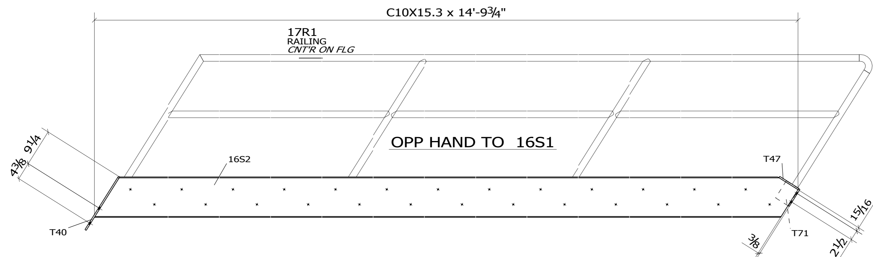
1 STRINGER(s) MARK: 16S2 >>> PER SPEC'S <<<
