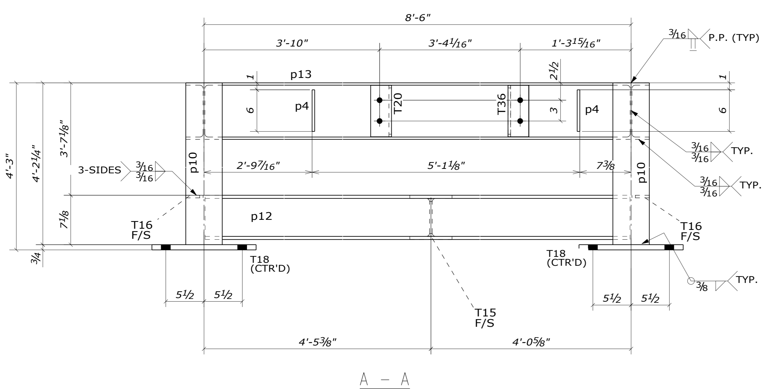
1 STAIR FRAME(S) MARK: 107A REF: D-08-C2096 HOT DIP GALV.
